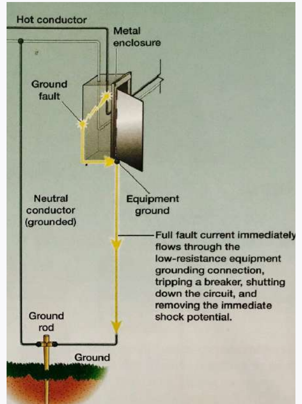
Figure 123: Proper Equipment Grounding
