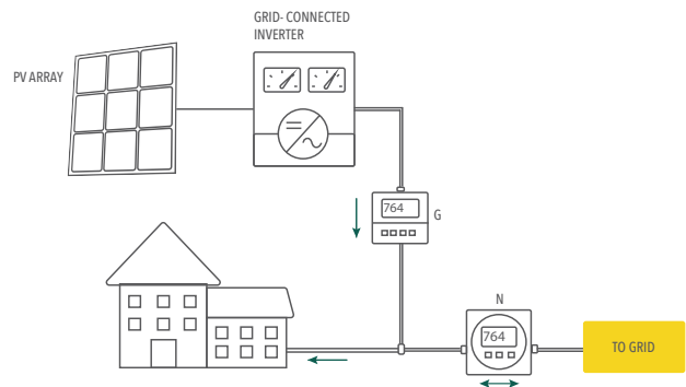
Figure 3: Grid connected PV System
