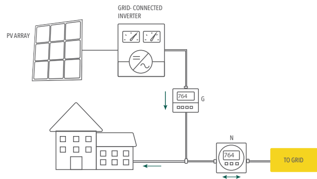
Figure 66: Grid-Connected Inverter
