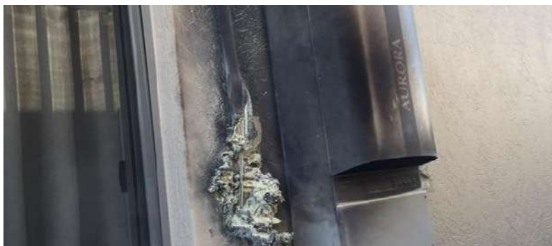
Figure 81: Inverter damage - Burn out
