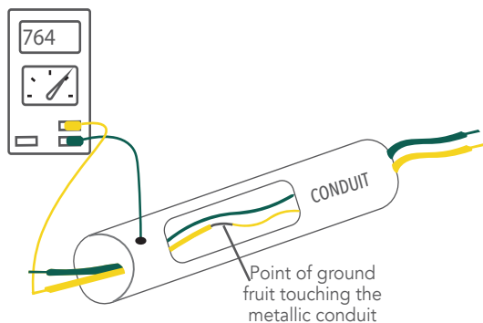
Figure 138: Continuity test
