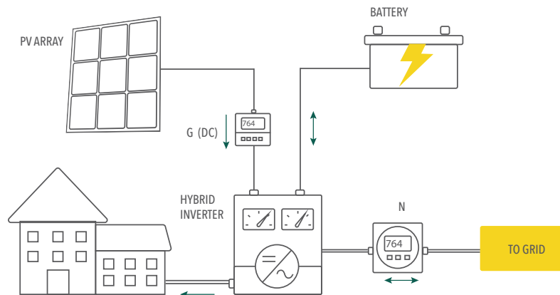
Figure 68: Hybrid Inverter
